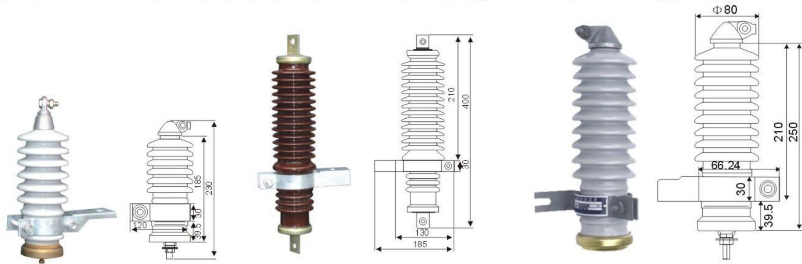
Fig.B61 Ur:3~6kV Creepage distance:280mm
